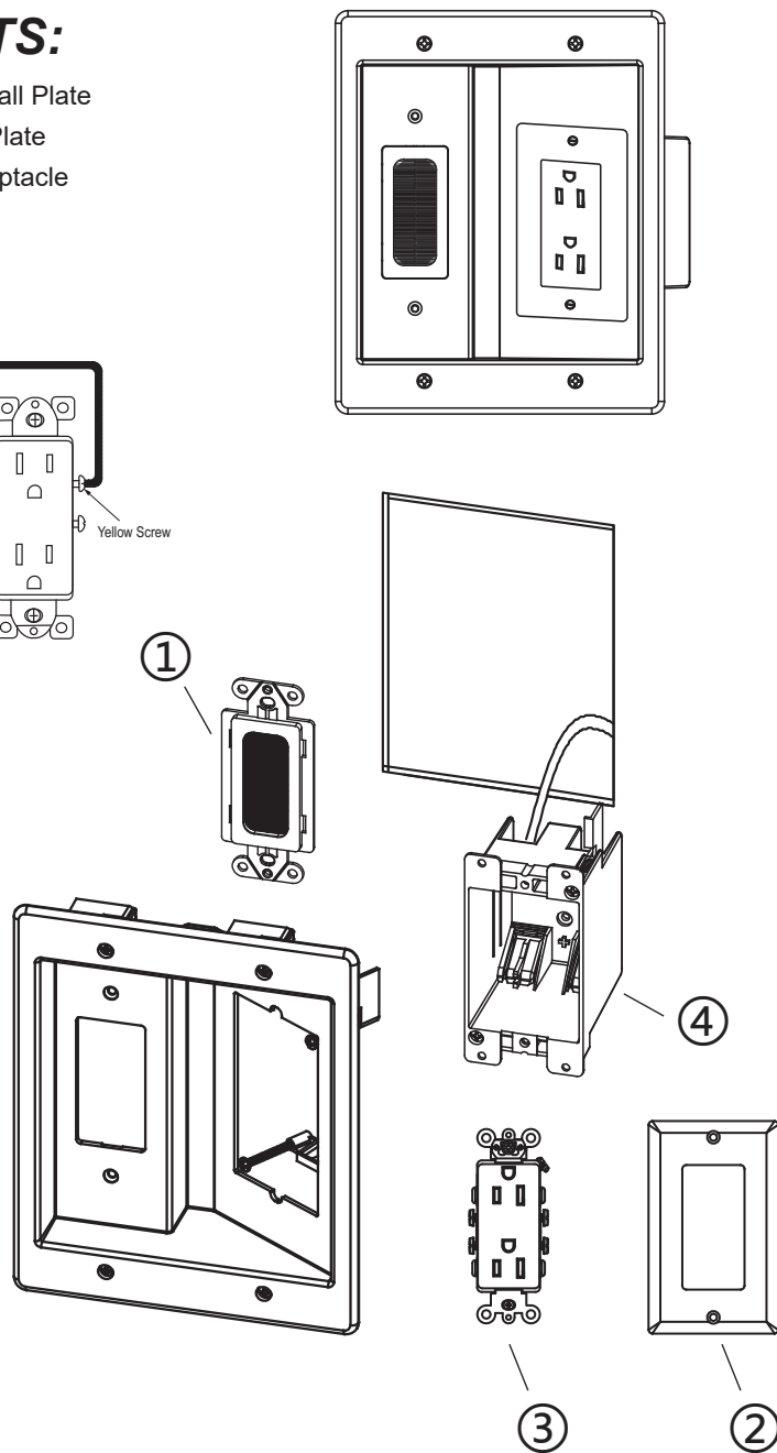
Installation Diagram
